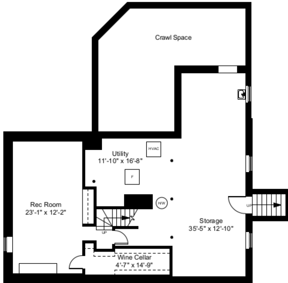
Lower Level Plan Ceiling Height = 7'-6"
